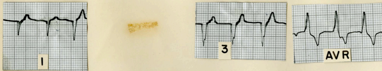
TRI-IODOETHYRONINE ACTIVITY
